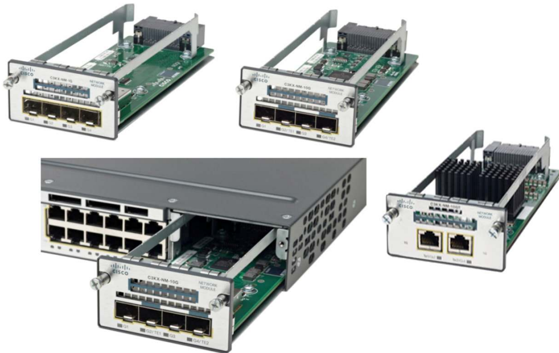
Figure 4. Network Module with Four GbE, Two 10GbE SFP+ Interfaces, Two 10GB-T and Service Module with Two 10GbE SFP+ Interfaces
